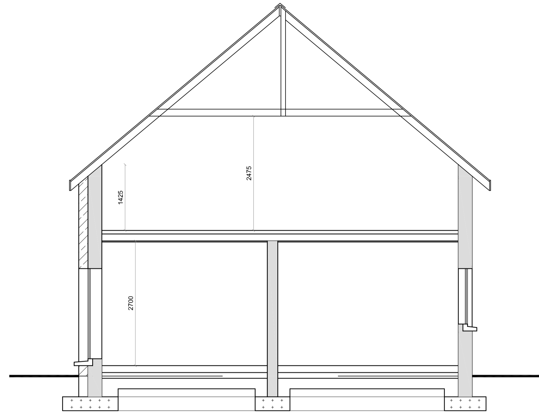
SECTION
